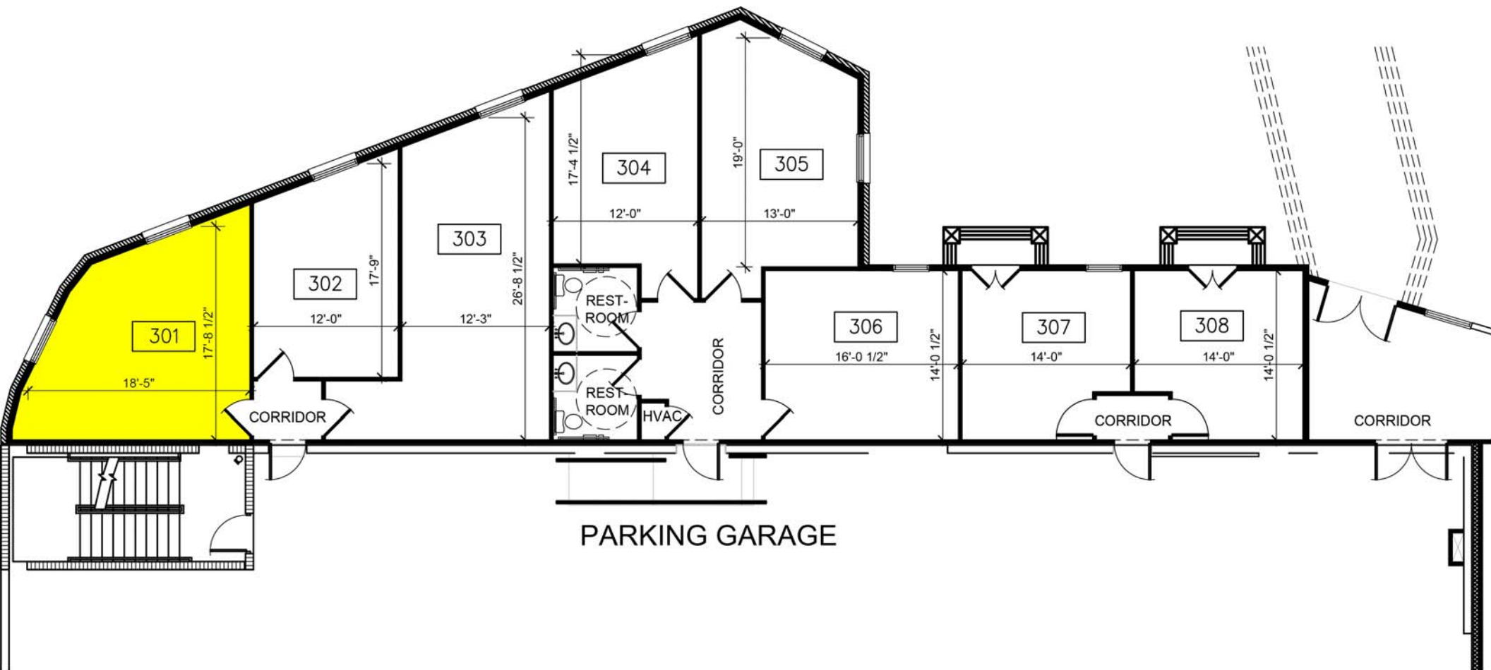
01 Third Floor Office Plan SCALE: 1/8" = 1'-0"
