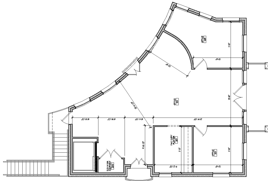
02 Second Floor Plan SCALE: 1/4" = 1'-0"
