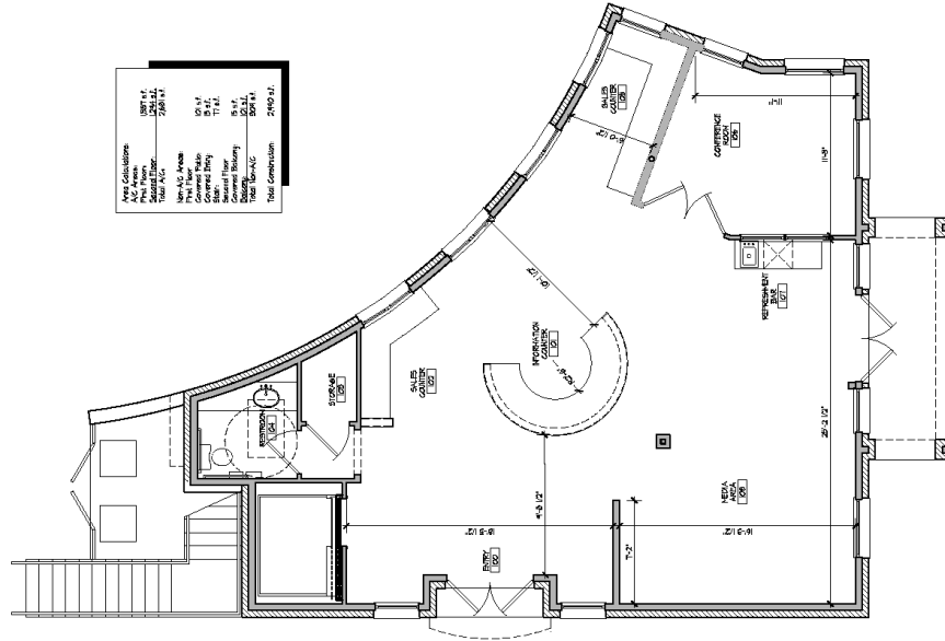
01 First Floor Plan SCALE: 1/4" = 1'-0"
