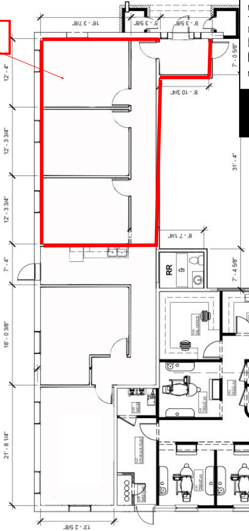
1 Floor Plan 1/8" = 1'-0"
